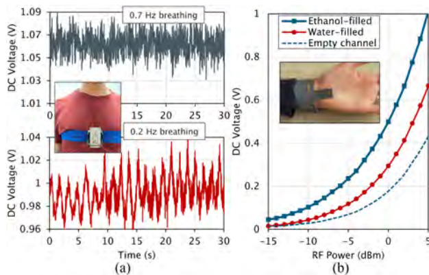
FIGURE 10. DC voltage-based readout of wearable microwave sensors: (a) SILO breathing sensor showing the breathing rate [127] (inset IEEE 2022); (b) ethanol-detection filter at different power levels [133] (inset IEEE 2021).
